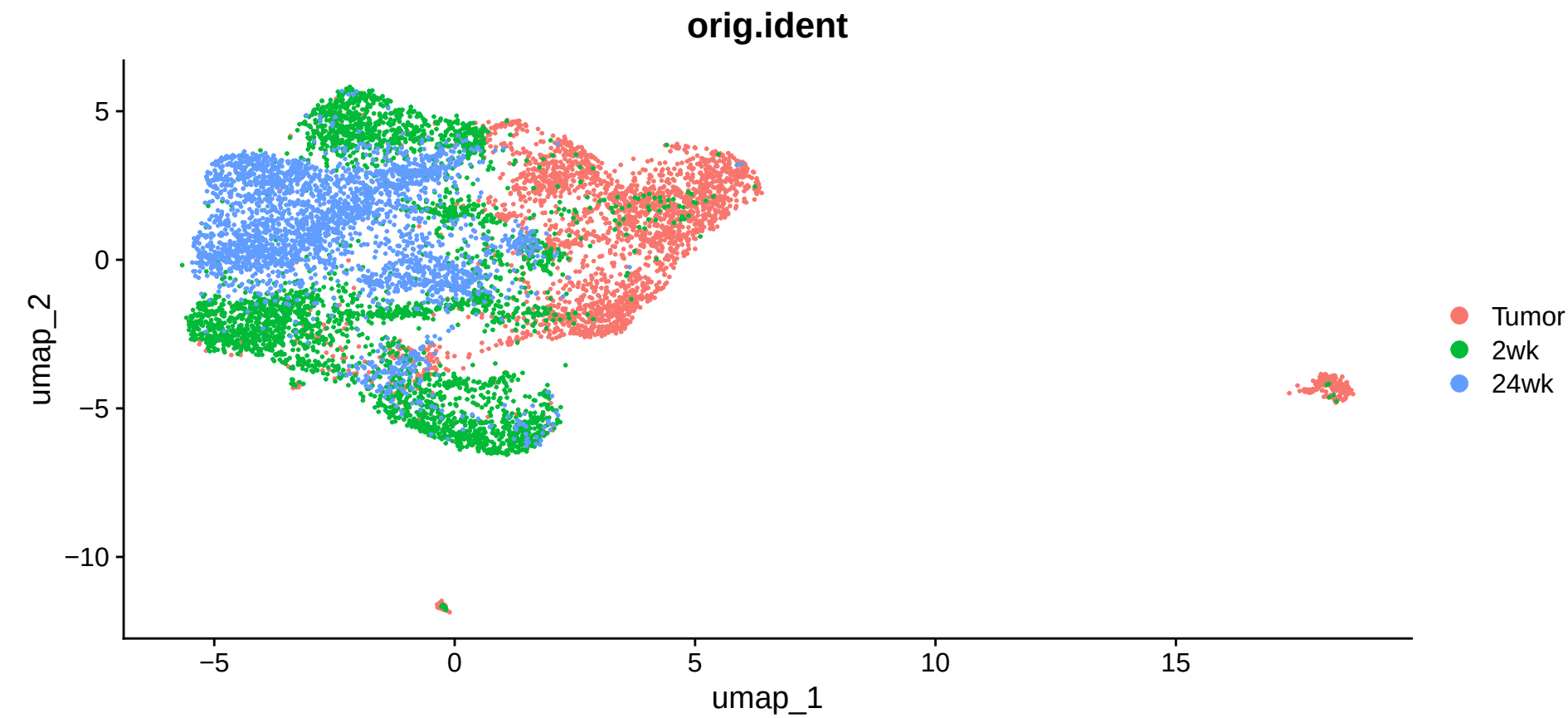
Before integration
