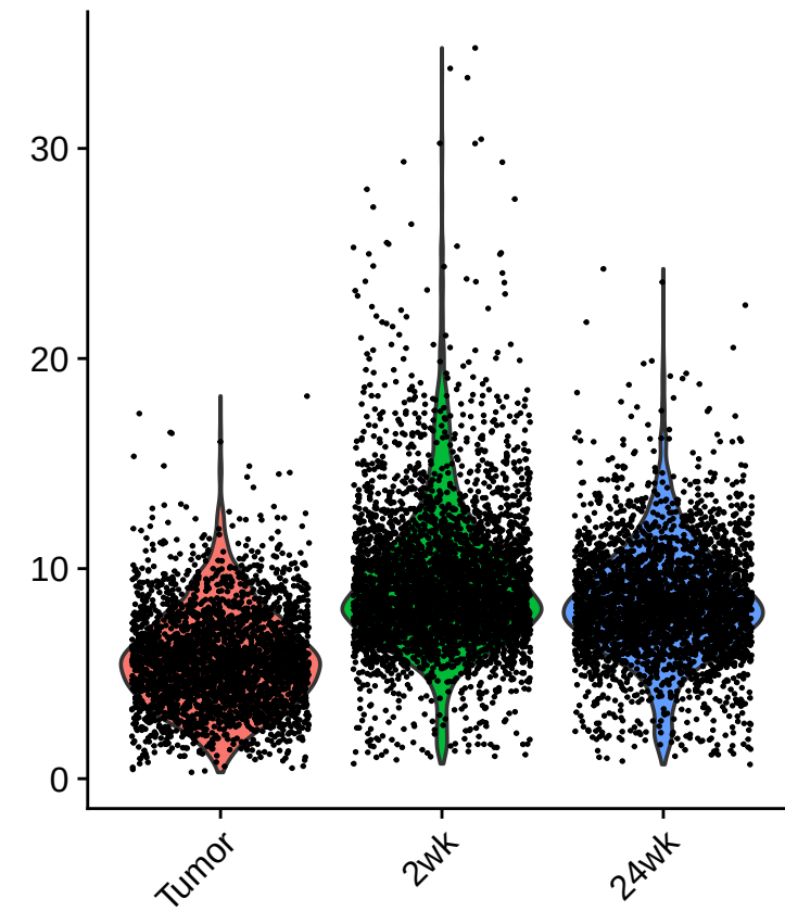
percent_ribo
