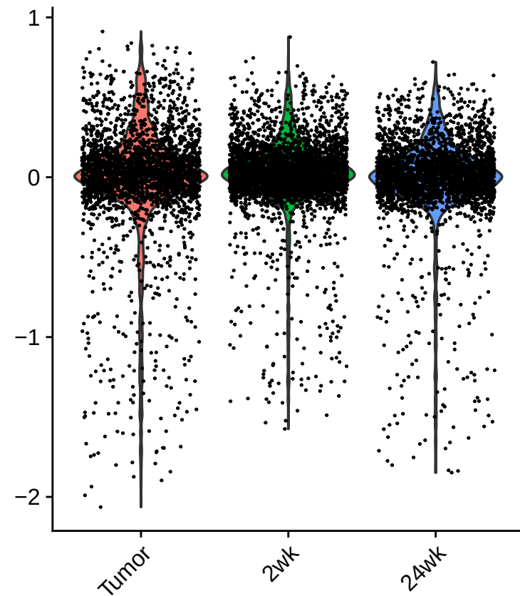
CC.Difference
