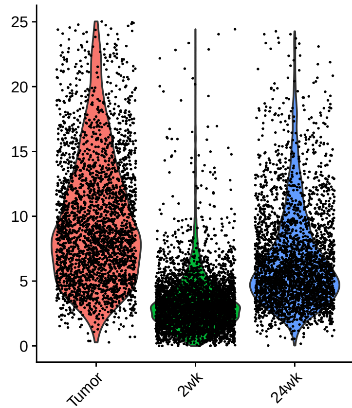
percent_mito
