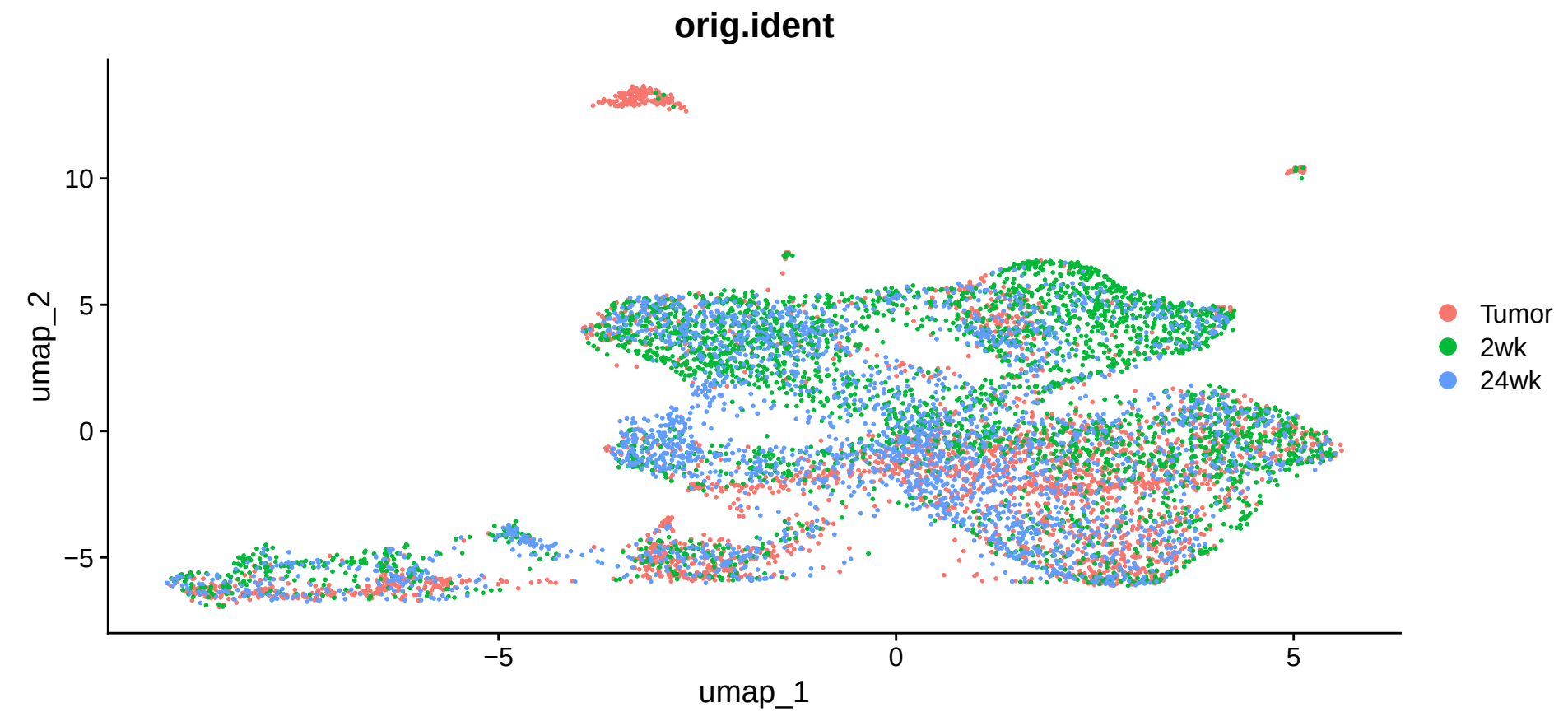
After integration
